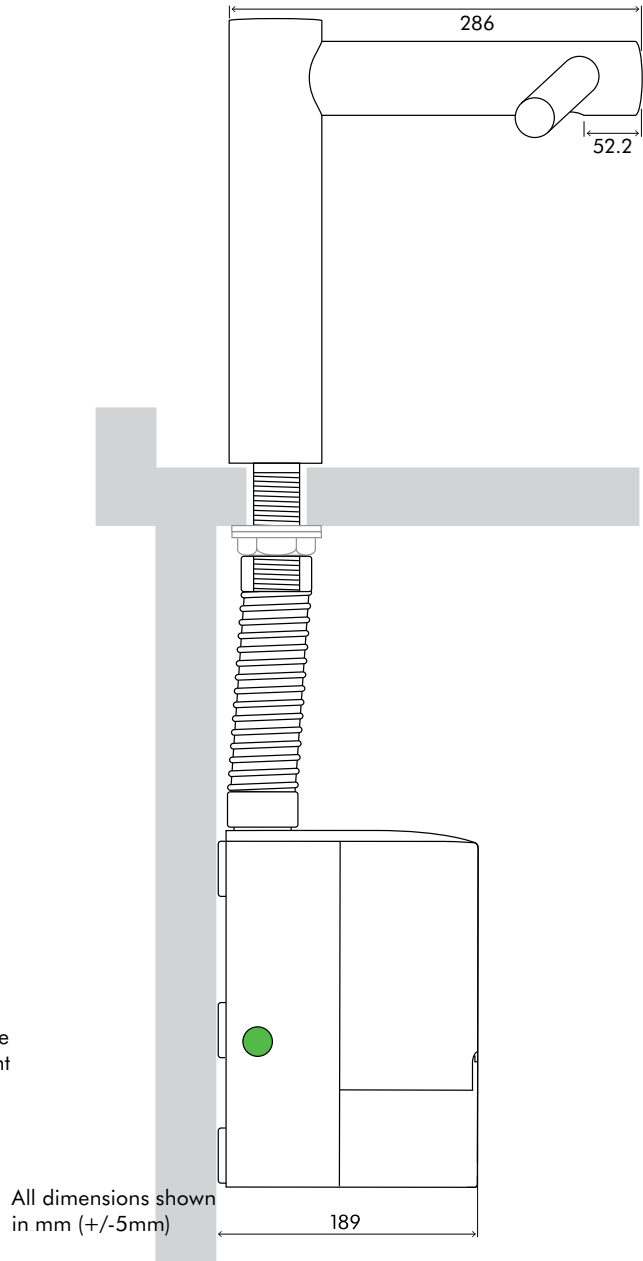
SIDE ELEVATION
