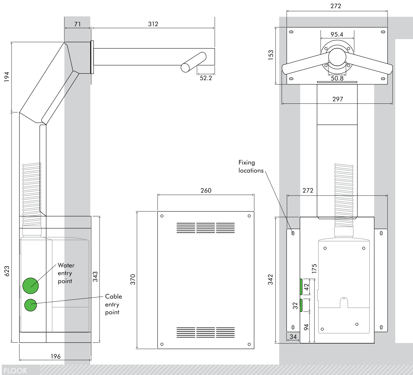
SIDE ELEVATION
